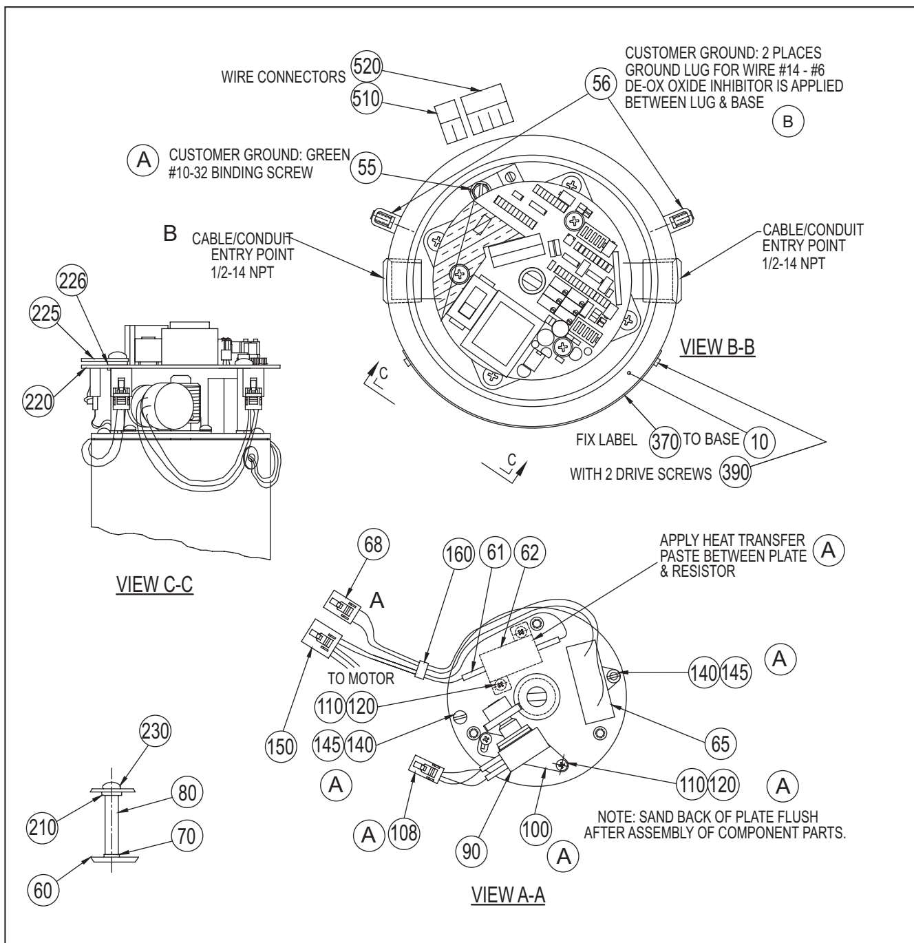
Figure 16C. Electronic Capacity Control (DWG 1022483000)
