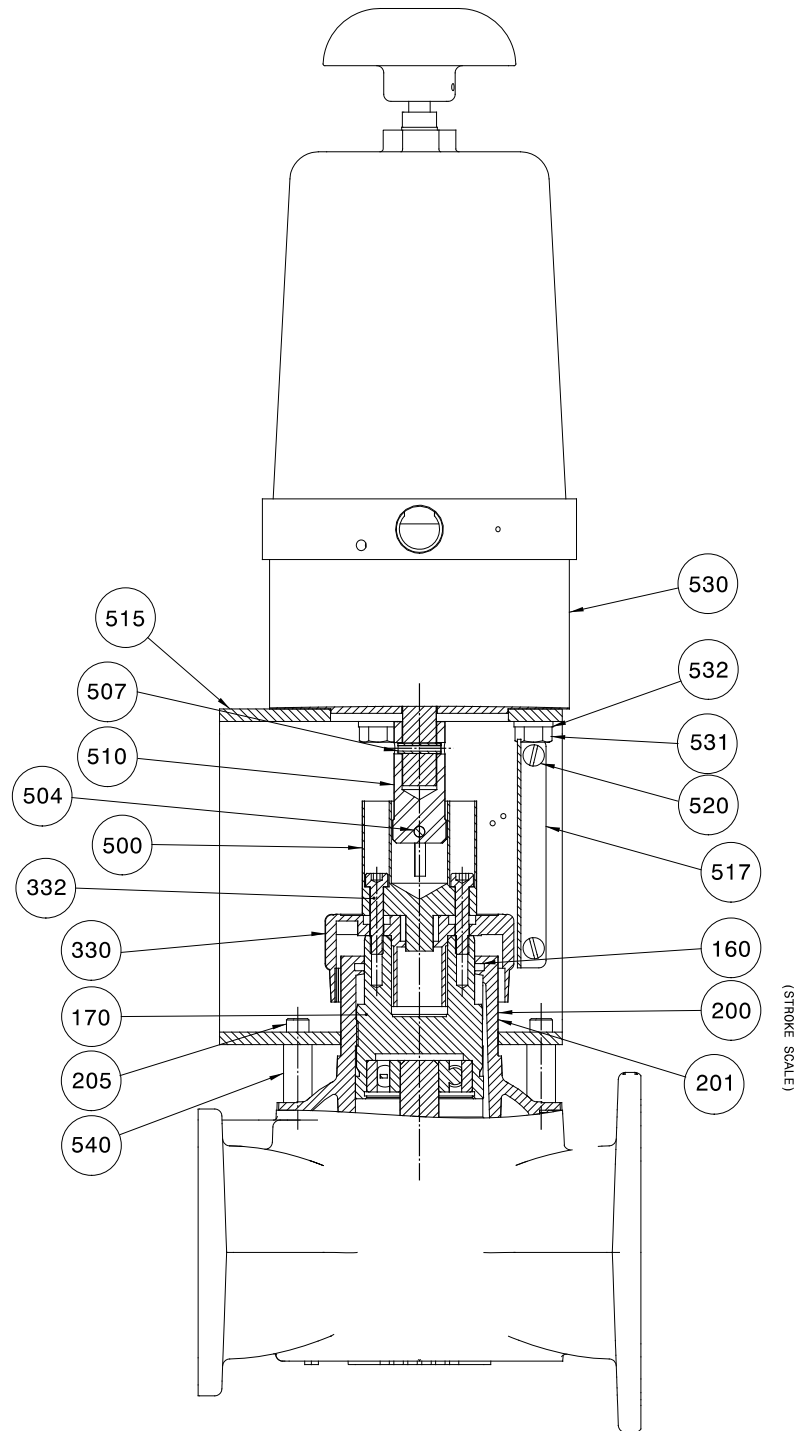
Figure 19B. (Sheet 2 of 2). MACROY® "D" ECC Mounting (DWG 1022728000)
