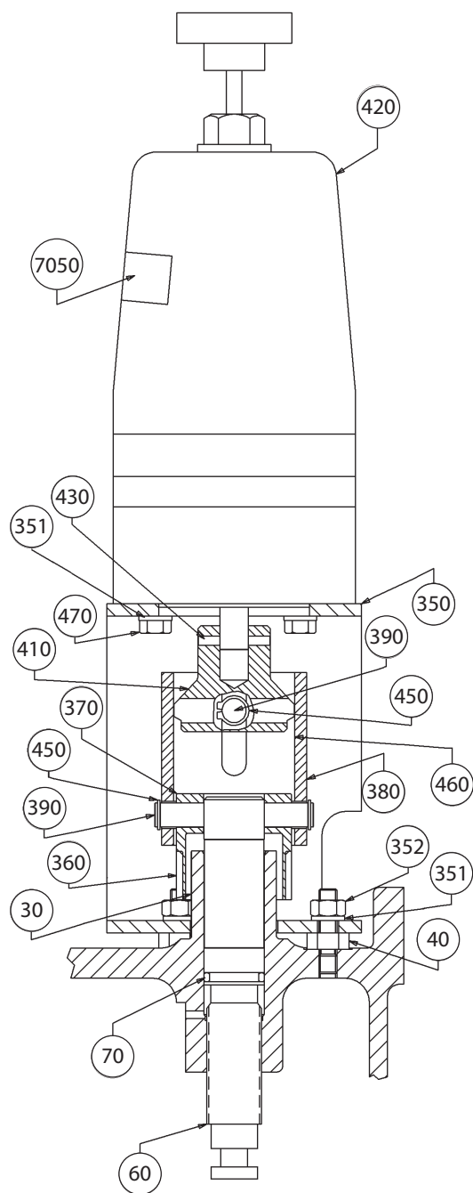
Figure 21A. (Sheet 1 of 2). Milroyal® B ECC Mounting Adapter (DWG 1022095000)
