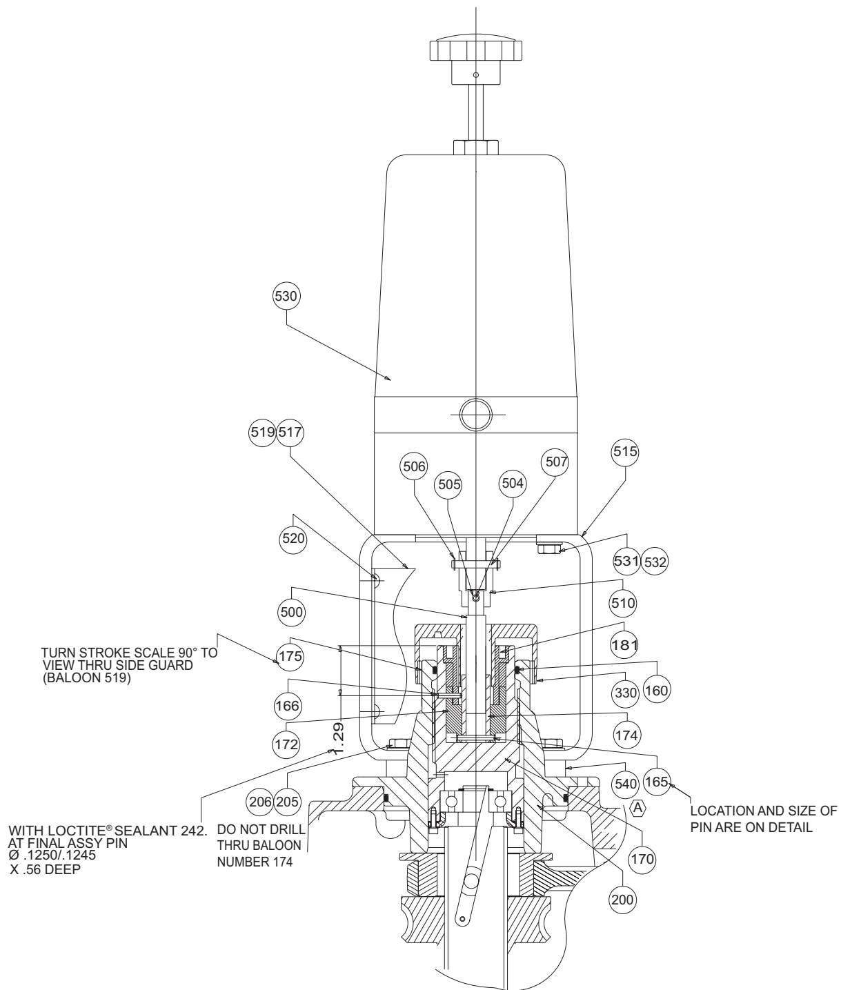
Figure 19A. (Sheet 1 of 2). MACROY® “G” ECC Mounting Adapter (DWG 1022118000) Design through “September 2004” and Milroyal® “G”.
