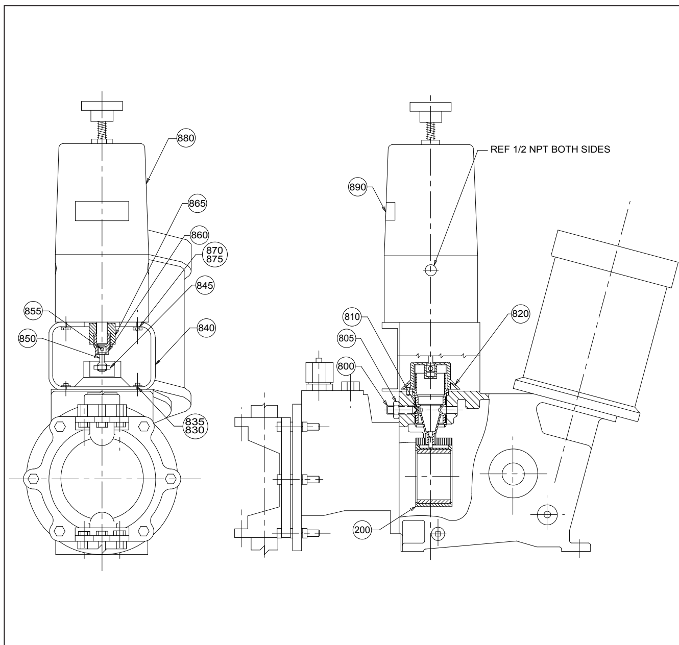
Figure 20. MAXROY® B ECC Mounting Adapter (DWG 1021572000).
