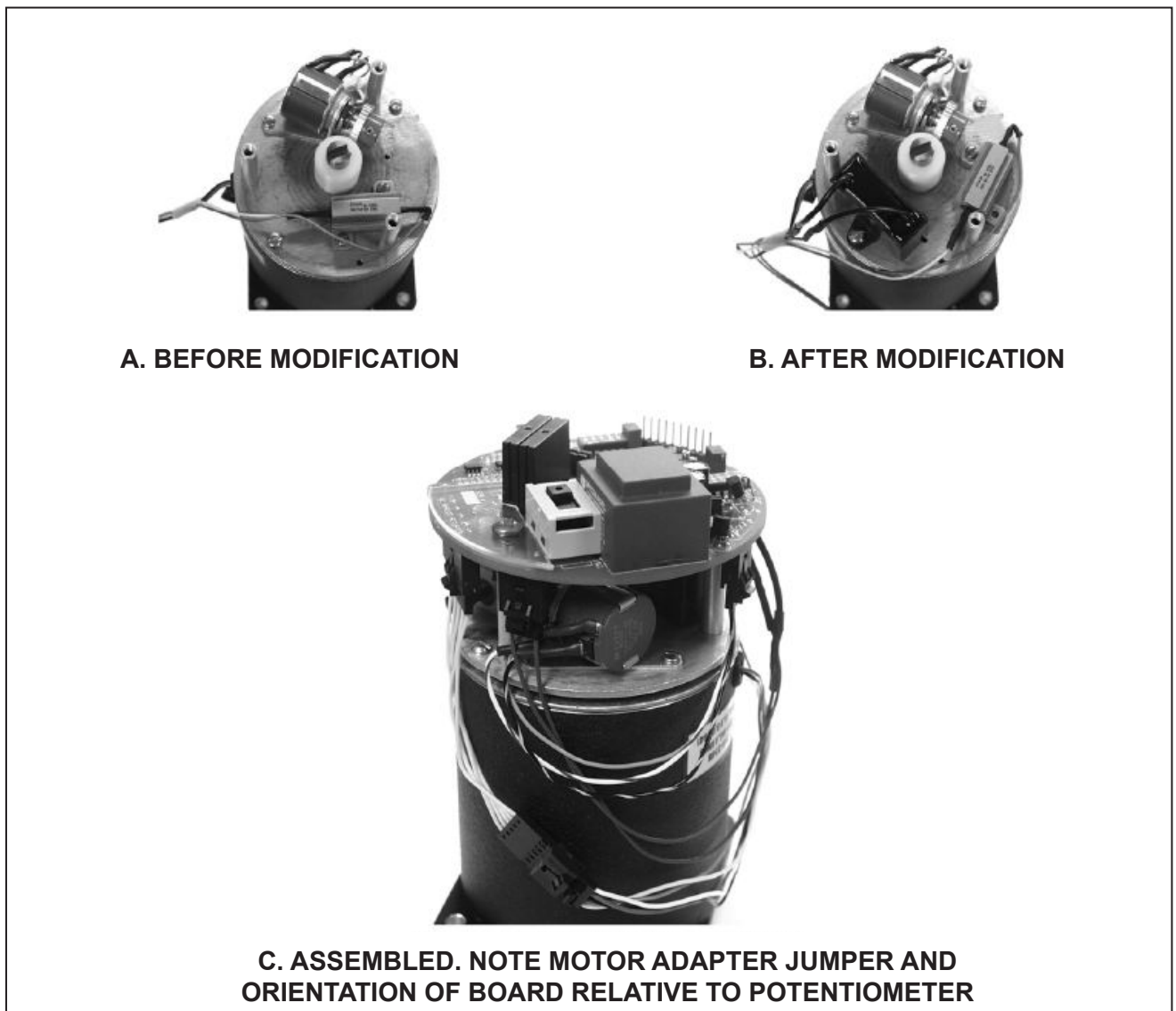
Figure 8. Conversion Detail
