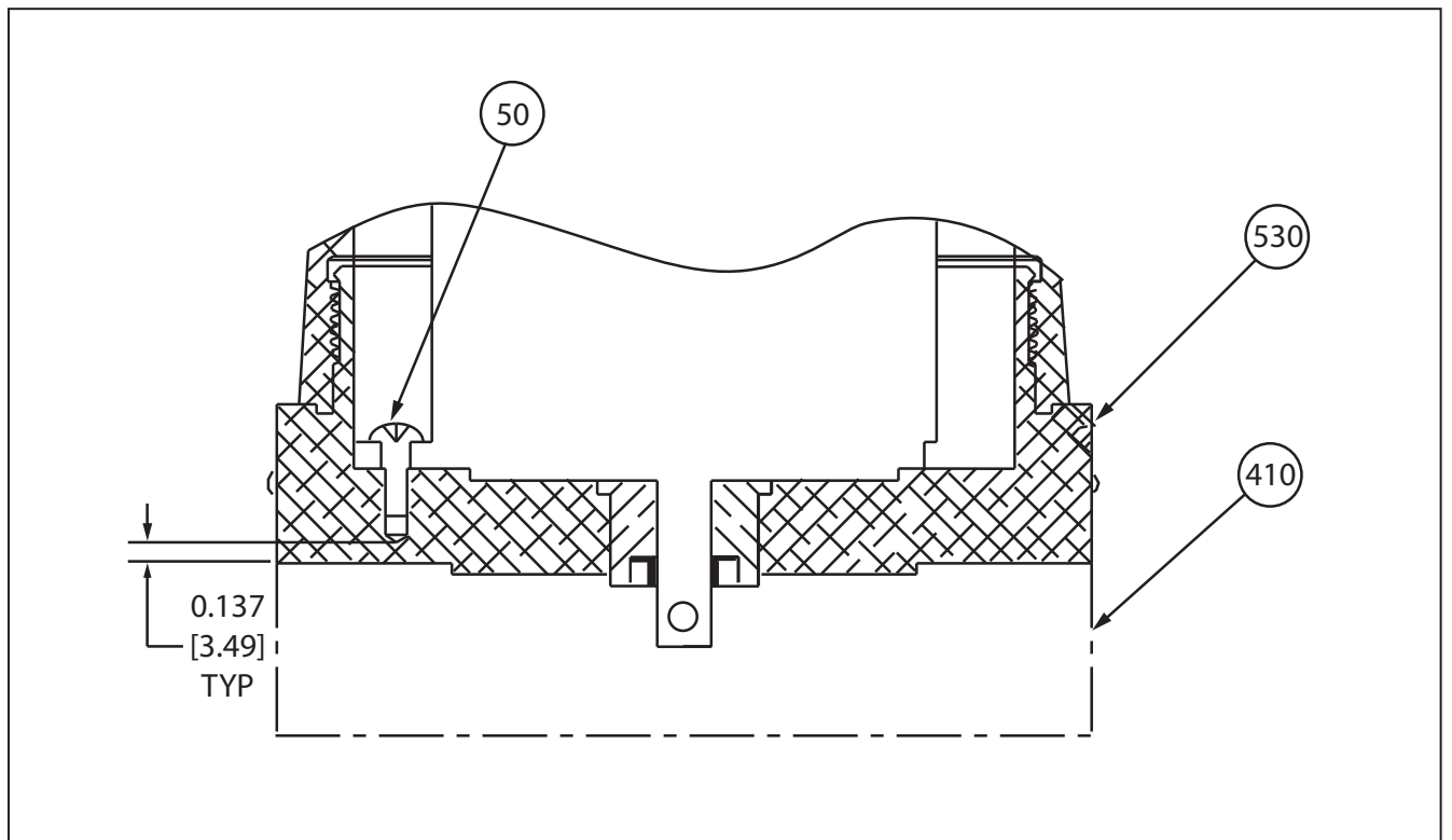
Figure 16B. Section B-B with Set Screw
