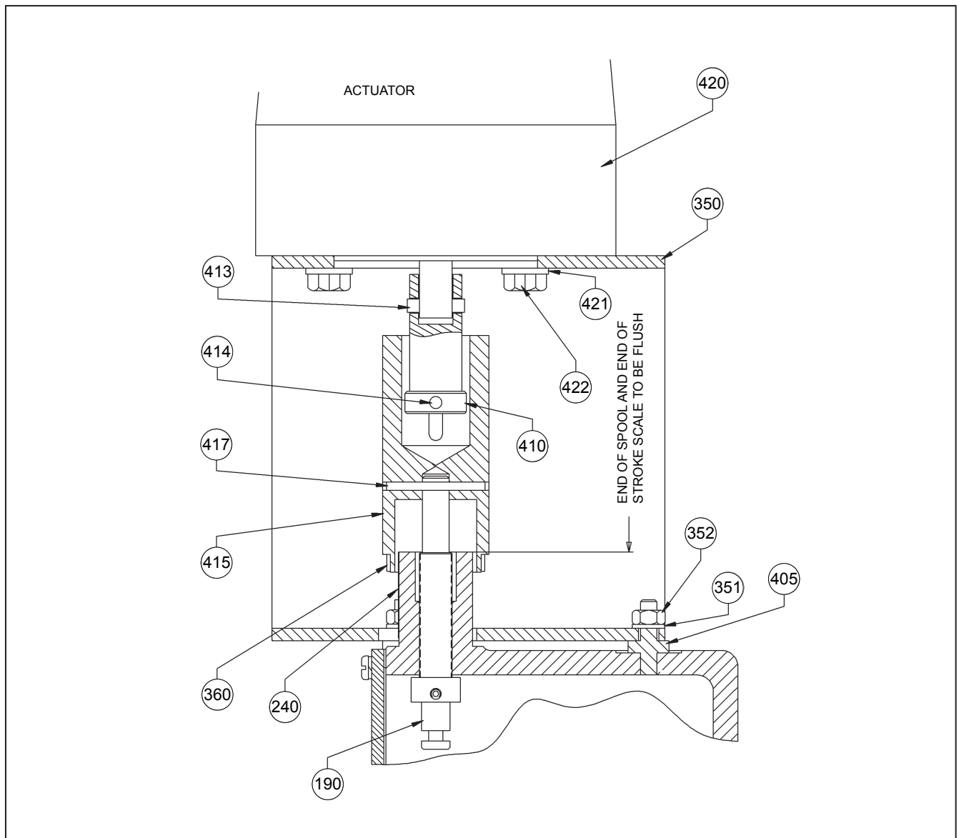
Figure 23. Milroyal® D ECC Mounting Adapter (DWG 1022906000)
