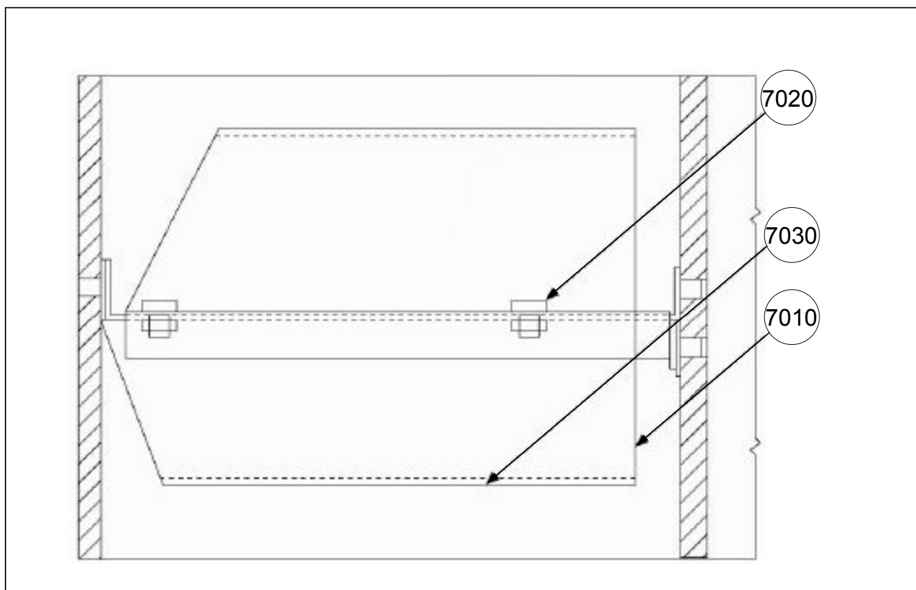
Figure 21B. (Sheet 2 of 2). Milroyal® B ECC Mounting Adapter Guard Assembly (DWG 1022095000)
