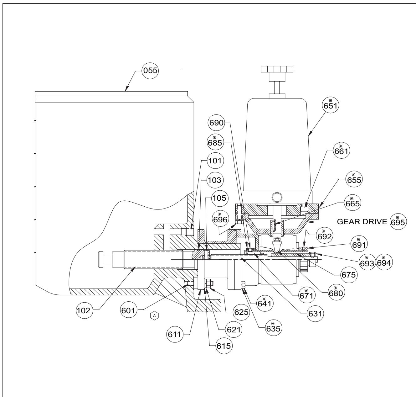
Figure 22. Milroyal® C ECC Mounting Adapter (DWG 10222850002)
