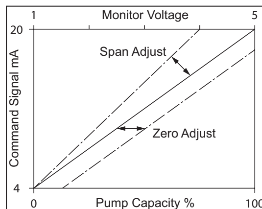
Figure 10. Effect of Zero & Span Controls
