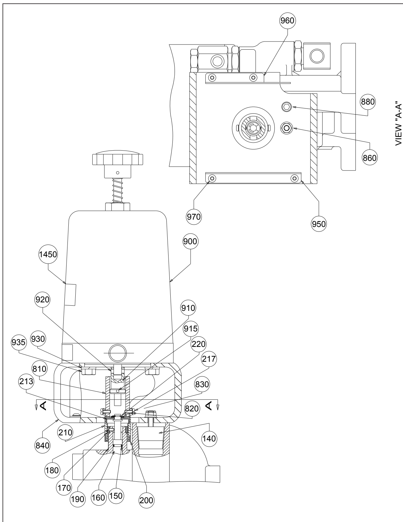
Figure 17. mRoy® "A" ECC Mounting Adapter (DWG 1021971000).
