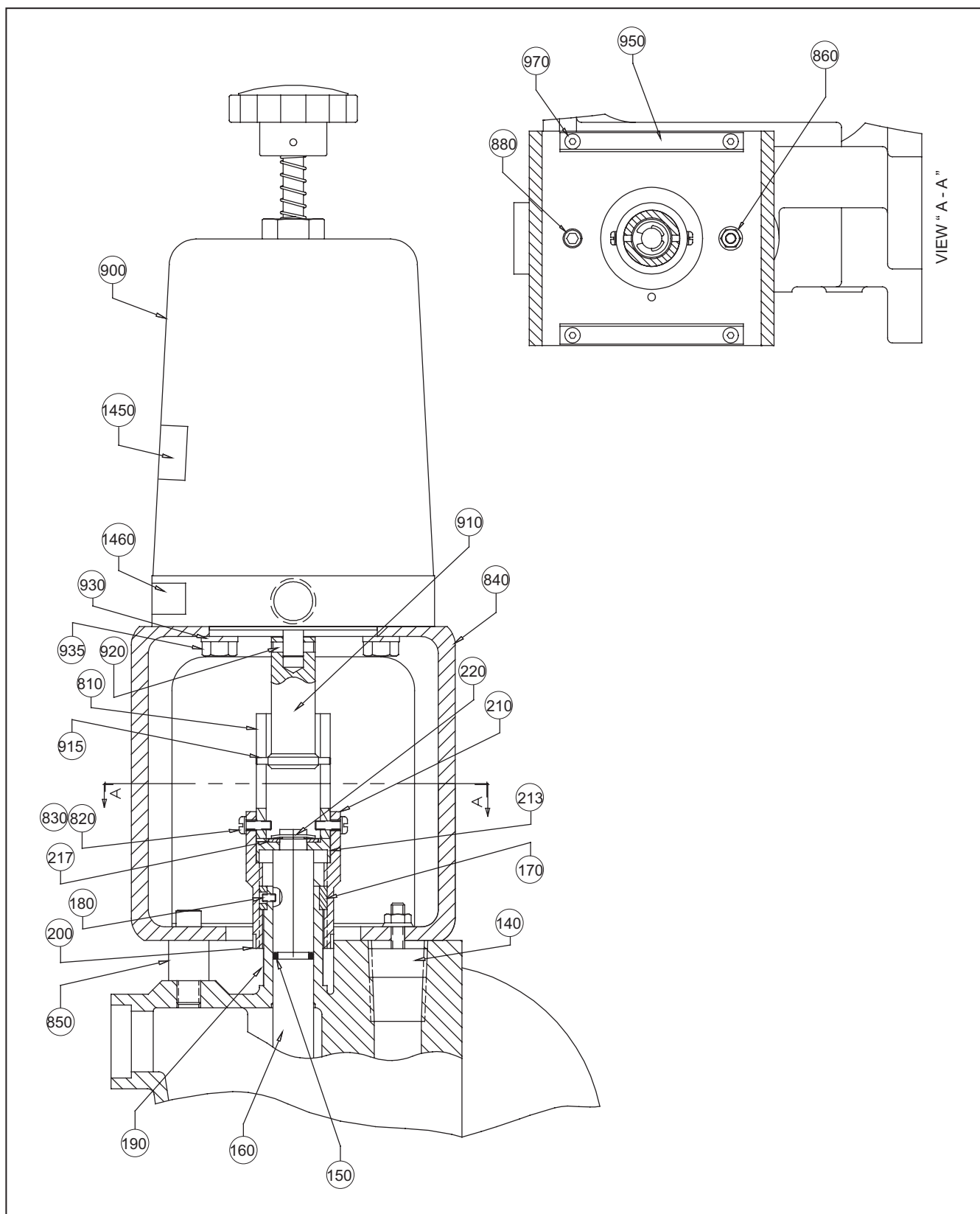
Figure 18. mRoy® "B" ECC Mounting Adapter (DWG 10221460003).
