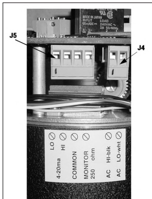
Figure 5. Circuit Board Connectors J4 and J5
