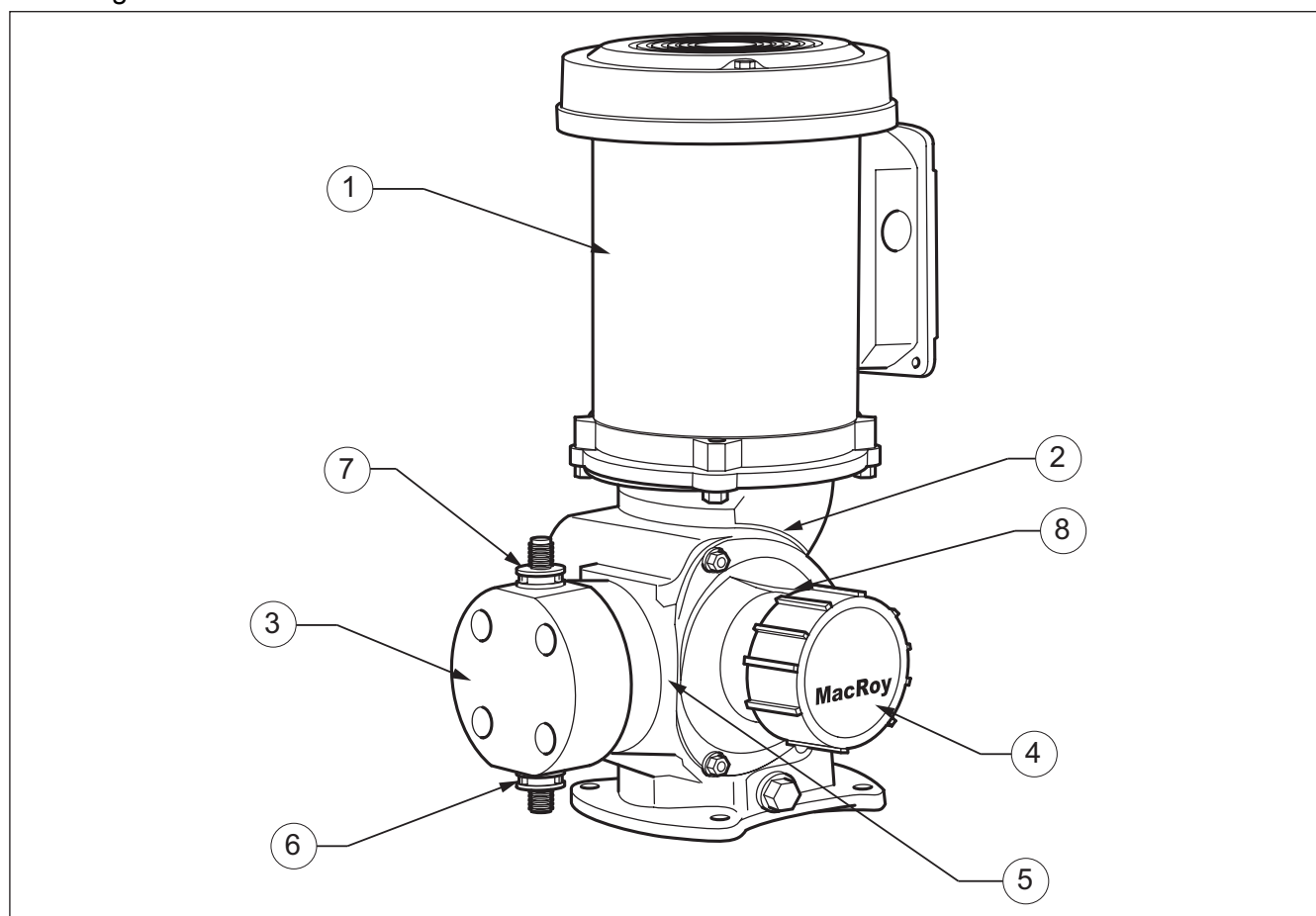
Figure 1. Pump Assembly
