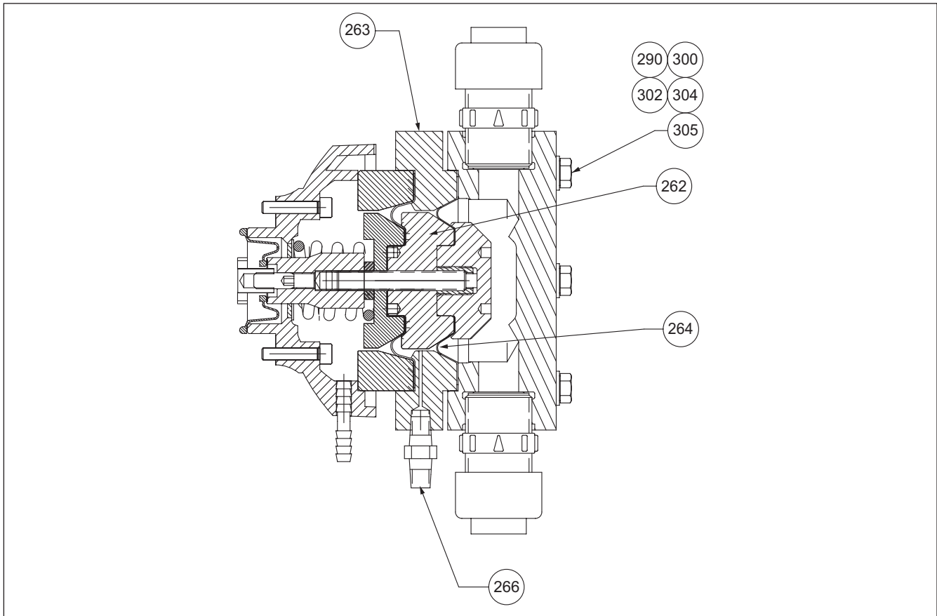
Figure 17. Double Diaphragm, D7 & D8 Pressure Type Configured (Optional) (102272800005)
