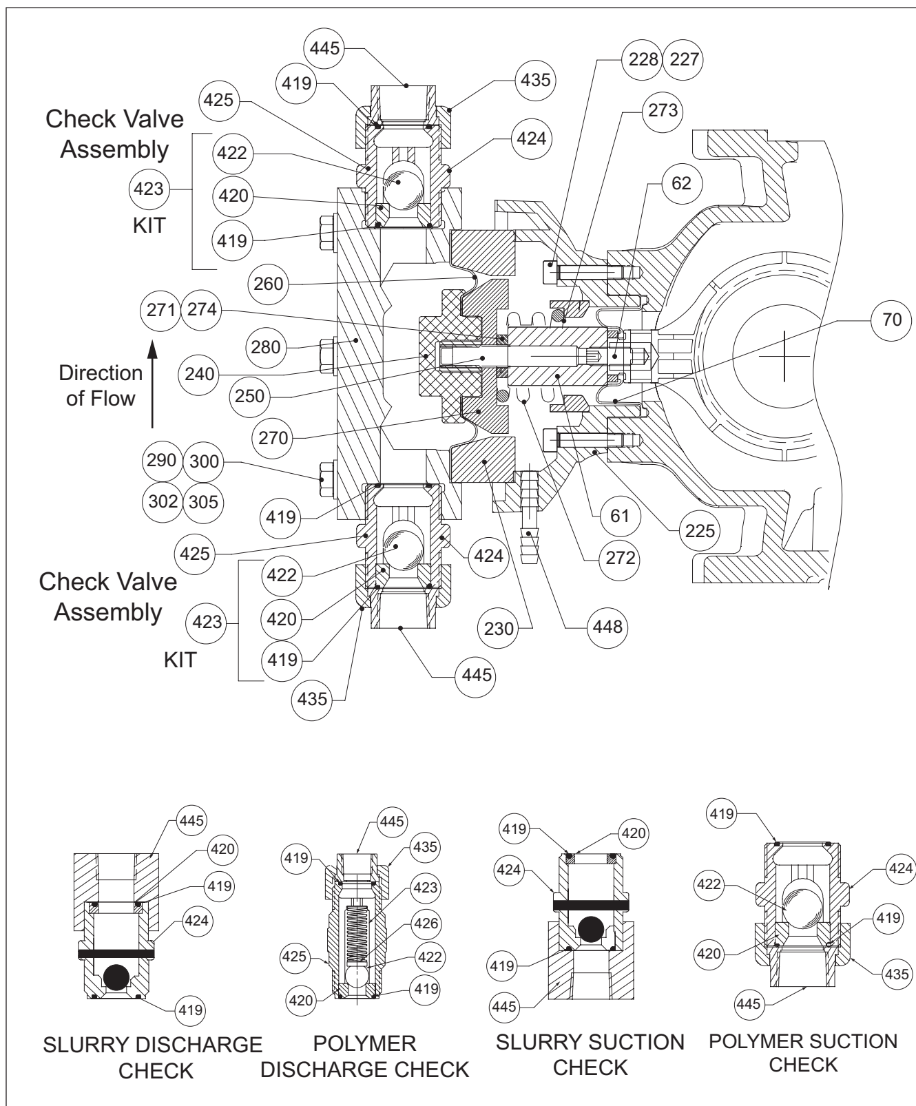
Figure 13. D7 & D8 Plastic Liquid End (1022819000)
