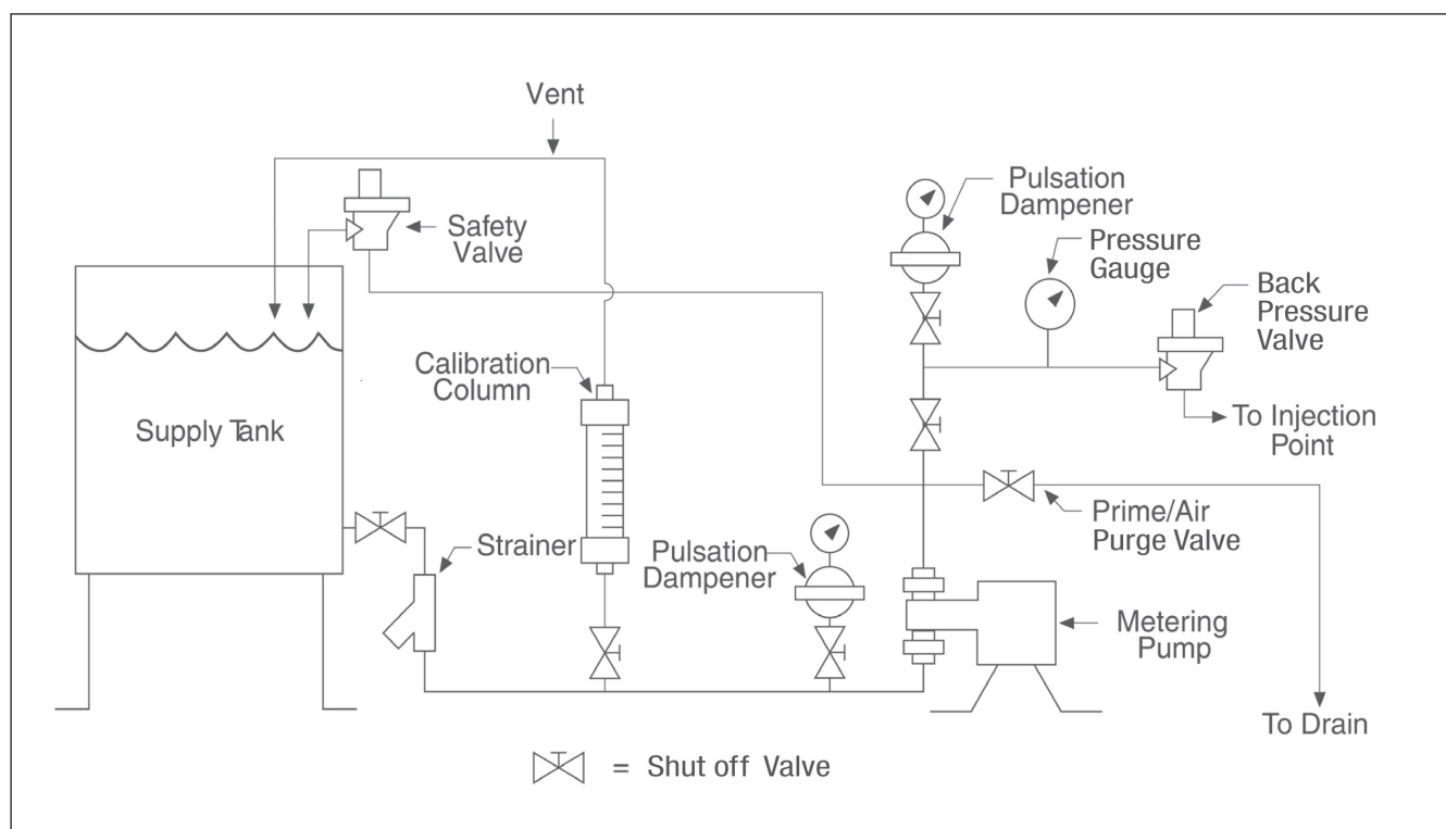
Figure 5. General Piping
