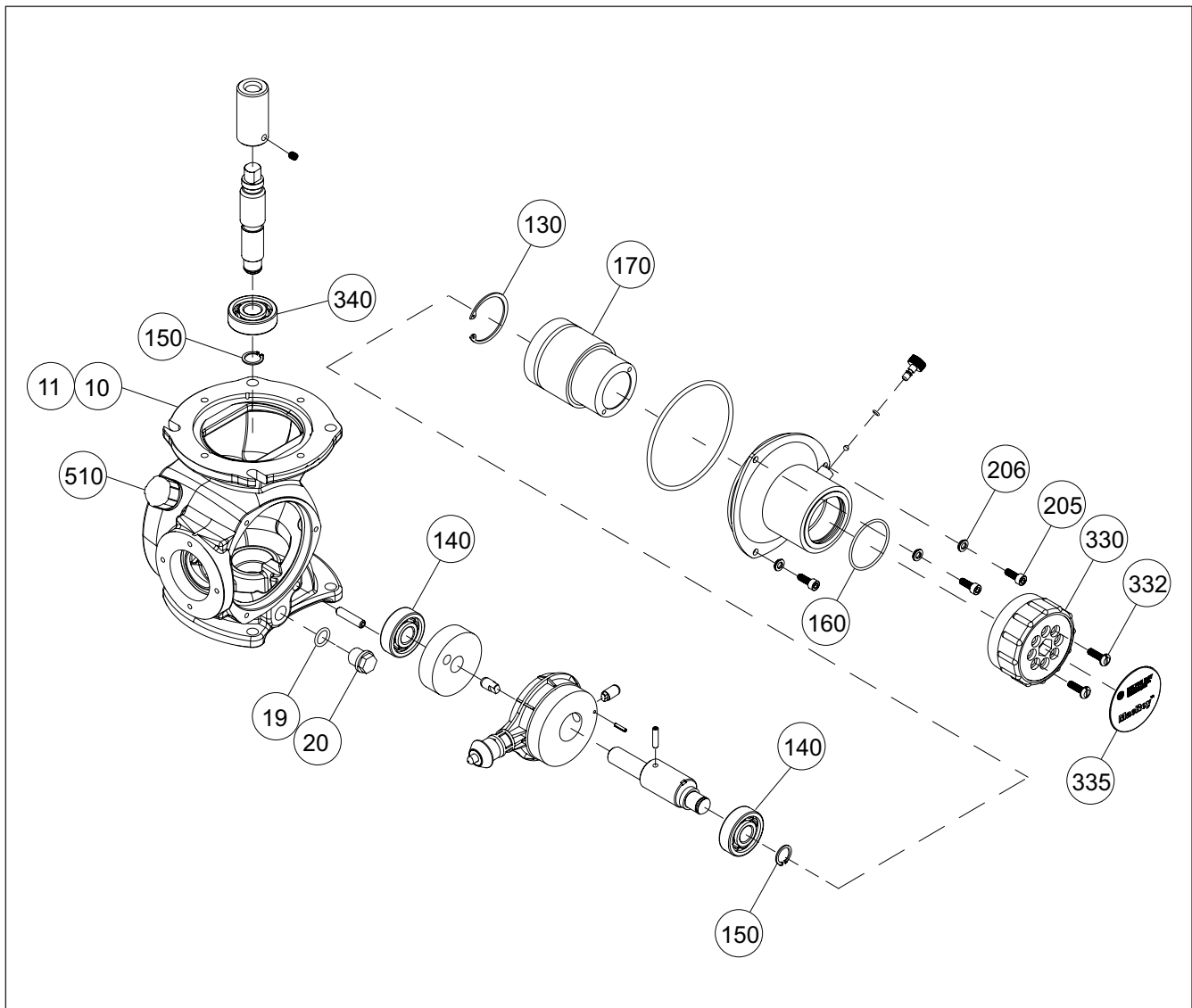
Figure 8. Drive Assembly (10227280007)
