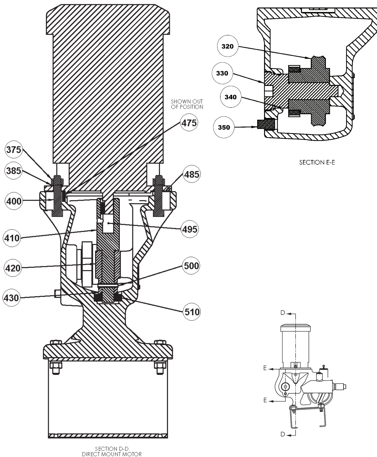
Figure 9. XT Direct Mount Motor / Mount / Gear Shaft (DWG 102-2633-000)
