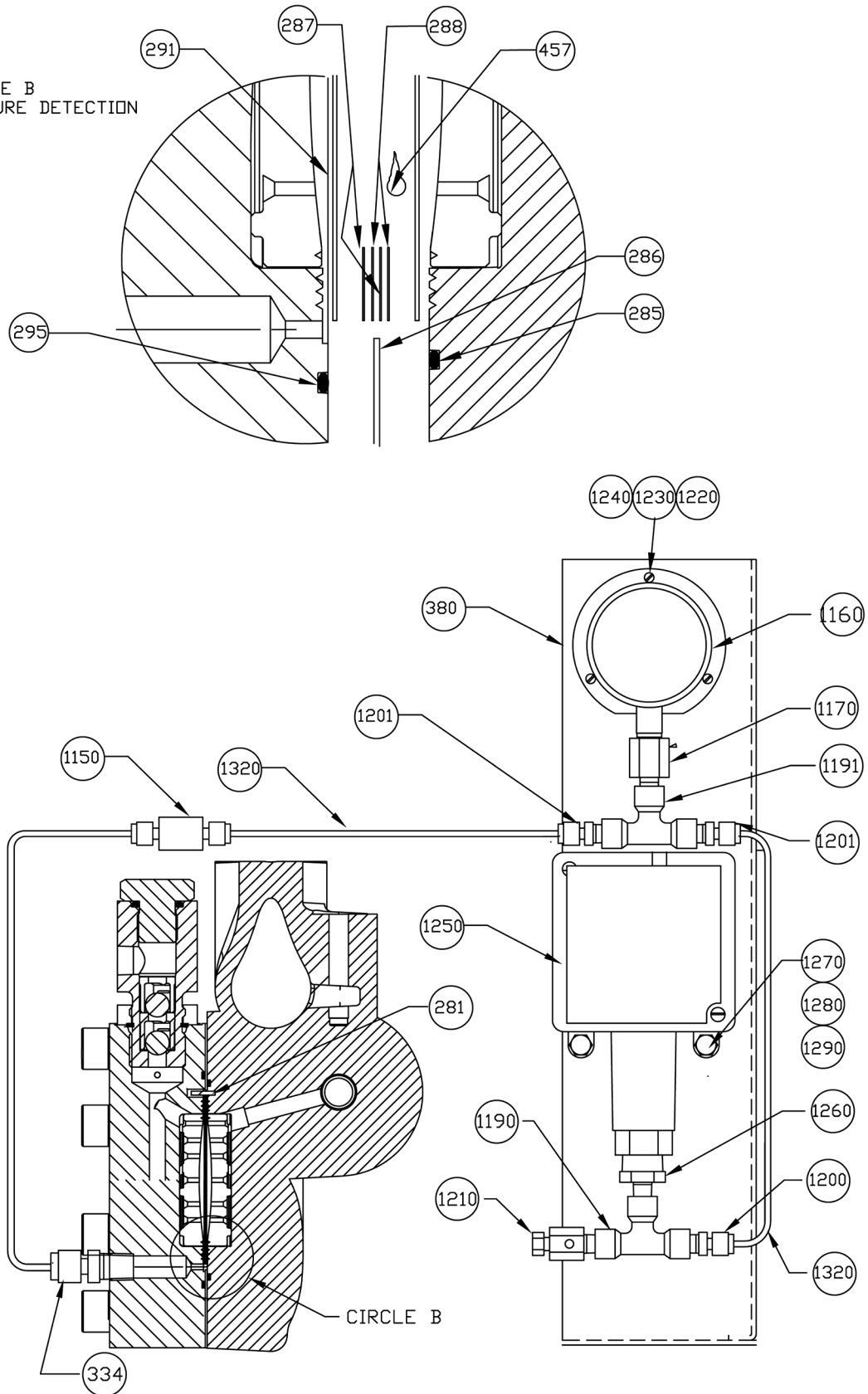
Figure 16. XW Liquid End With Rupture Detection (Sheet 1 of 2) (DWG 102-2402-000)
