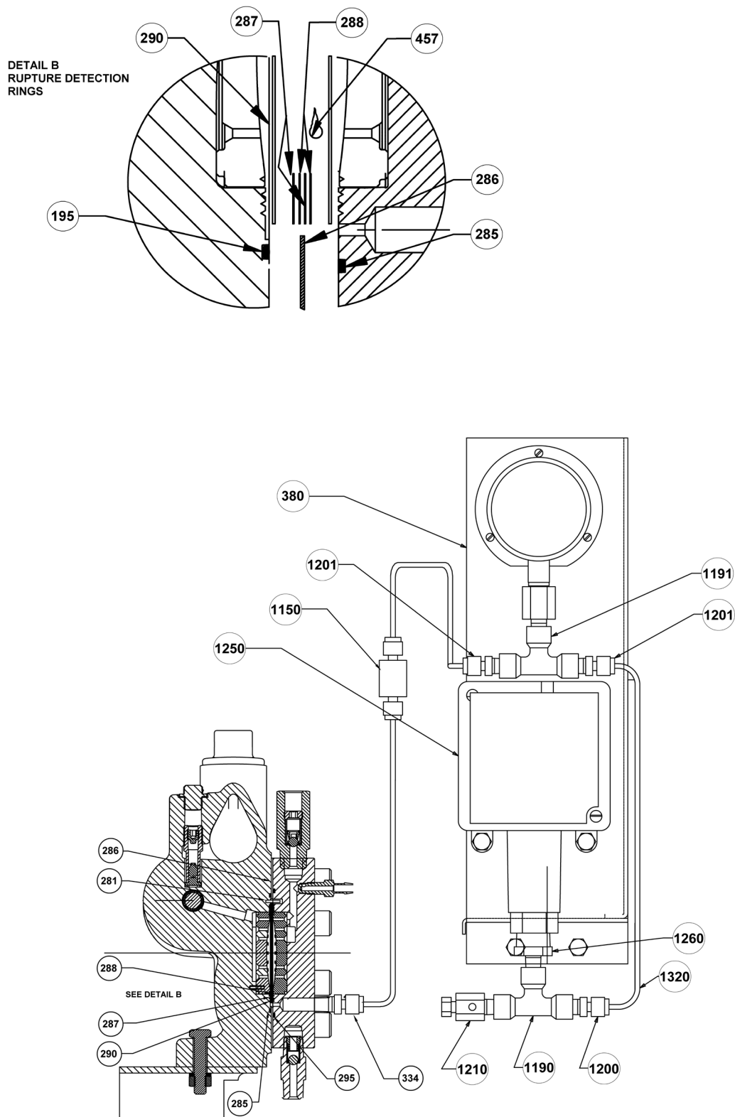
Figure 12. XT With Rupture Detection (Sheet 2 of 2) (DWG 102-2633-000)
