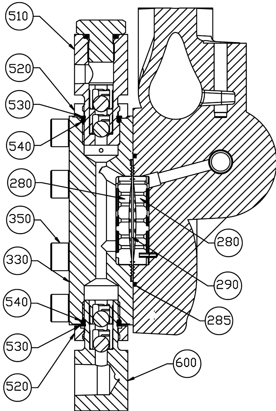
Figure 16. Additional Rupture Detection Parts (Sheet 2 of 2) (DWG 102-2402-000)
