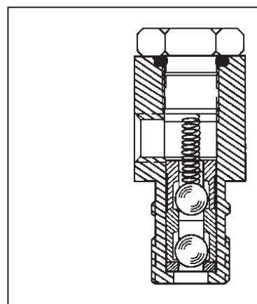
Figure 5. Back Pressure Spring Installation
