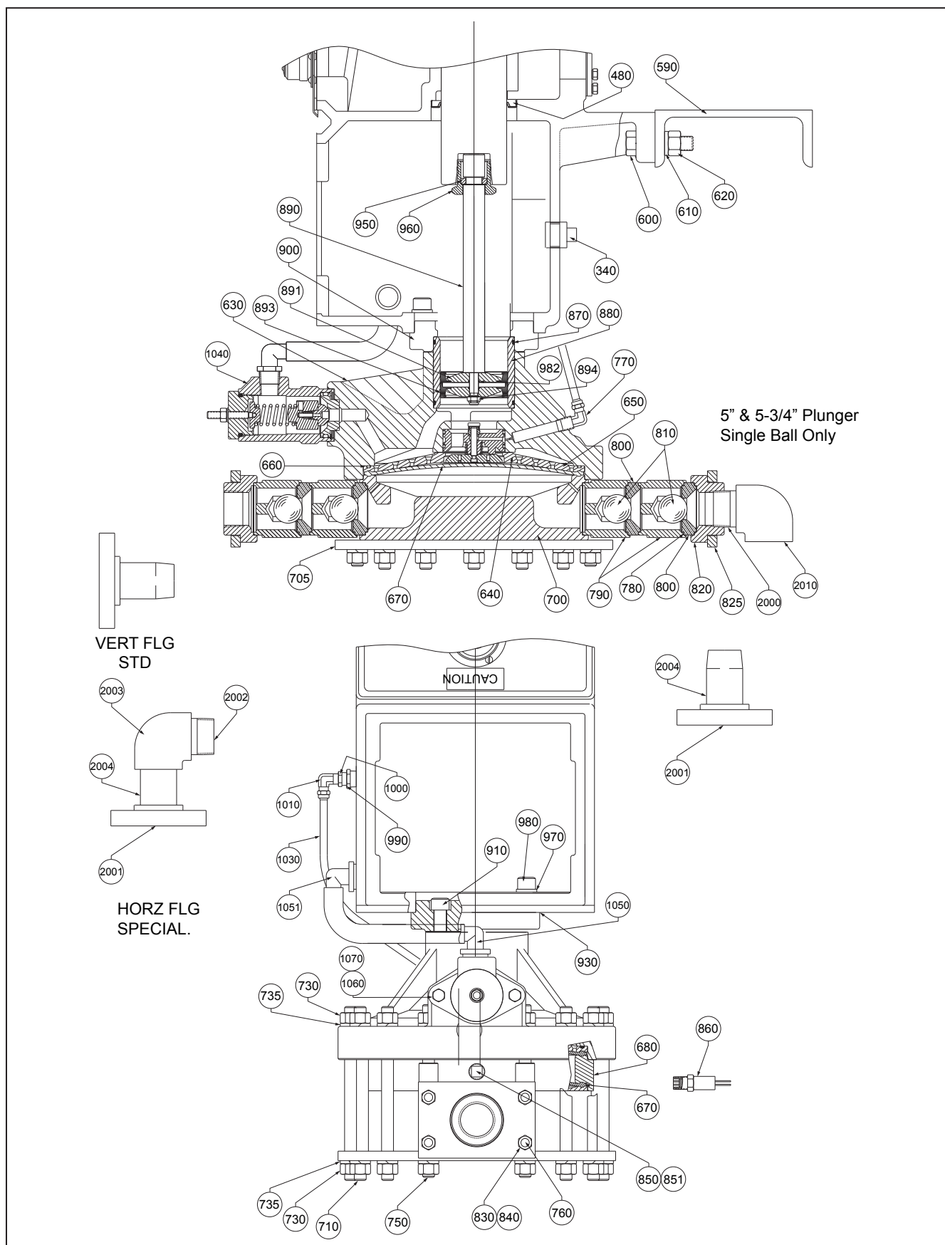
Figure 11. Milroyal® C, HPD Plastic Liquid End Assembly (DWG. 102-2285-000 Sheet 5)
