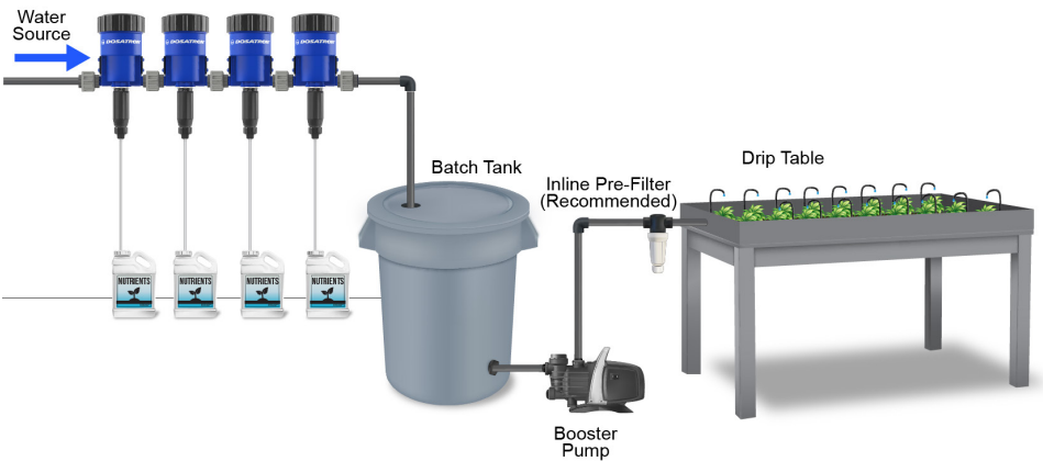
Figure 6 - Batch Tank Illustration
