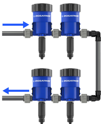
Figure 3 - U-Shape Configuration
