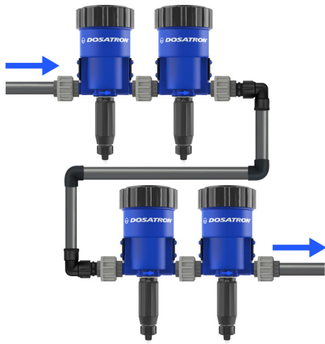
Figure 4 - Serpentine Configuration
