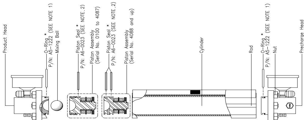
DURASITE EXPLODED VIEW
