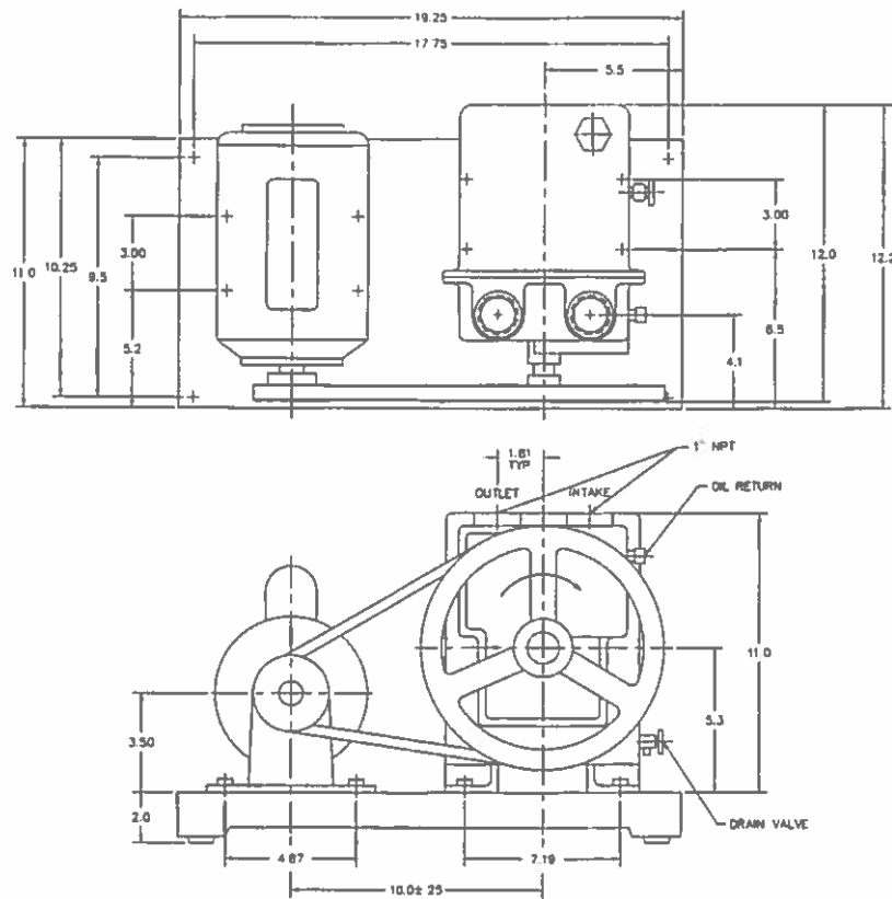
CRR-1A and CRR-1B Dimensional Diagram
