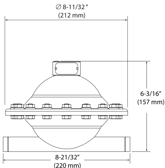
SBA05S-ASS-TA (ACTIVE, 1/2" NPT THREAD - HORIZONTAL)
