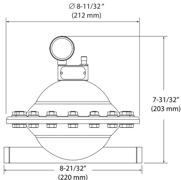
SBP05S-ASS-TA (PASSIVE, 1/2" NPT THREAD - HORIZONTAL)
