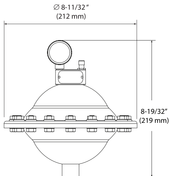
SBP05S-LSS-TA (PASSIVE, 1/2" BSP THREAD - VERTICAL)
