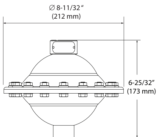
SBA10S-LSS-TA (ACTIVE, 1" BSP THREAD - VERTICAL) SBA10S-OSS-TA (ACTIVE, 1" NPT THREAD - VERTICAL)
