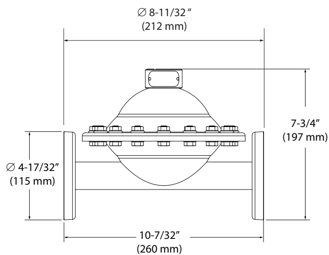
SBA105-FSS-TA (ACTIVE, 1" FLANGE - HORIZONTAL)
