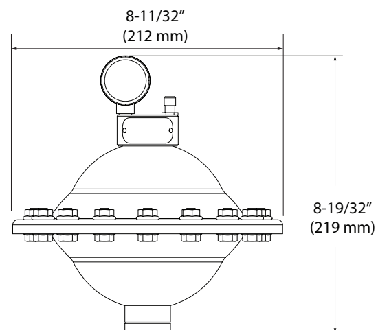
SBP10S-LSS-TA (PASSIVE, 1" BSP THREAD - VERTICAL) SBP10S-OSS-TA (PASSIVE, 1" NPT THREAD - VERTICAL)
