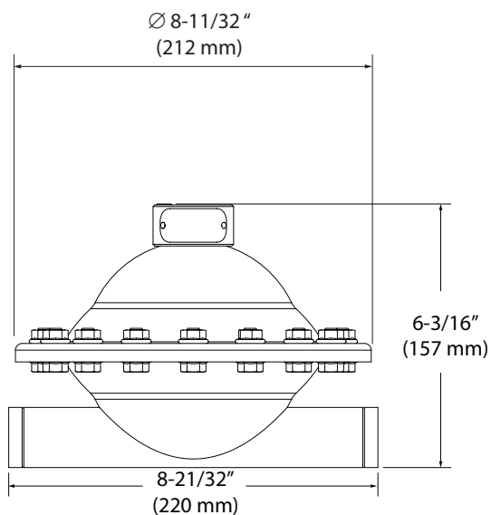
SBA10S-ASS-TA (ACTIVE, 1" NPT THREAD - HORIZONTAL) SBA10S-BSS-TA (ACTIVE, 1" BSP THREAD- HORIZONTAL)
