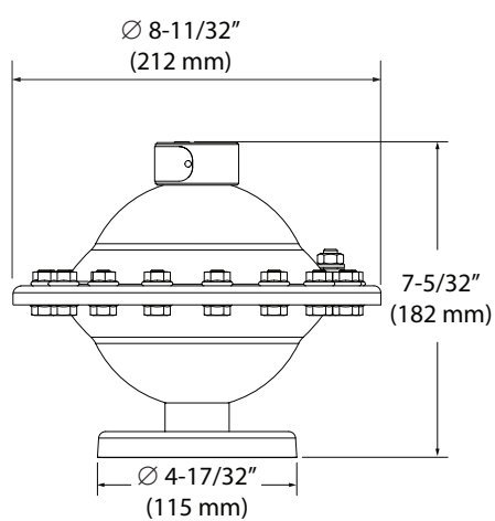
SBA105-ESS-TA (ACTIVE, 1" FLANGE - VERTICAL)
