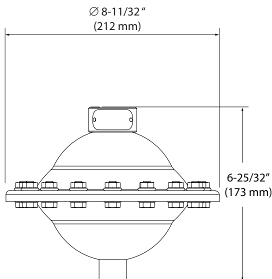
SBA05S-LSS-TA (ACTIVE, 1/2" BSP THREAD - VERTICAL)
