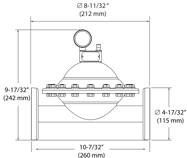
SBP105-FSS-TA (PASSIVE, 1" FLANGE - HORIZONTAL)
