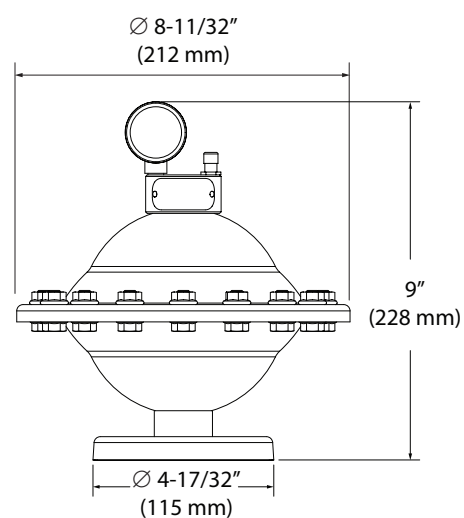
SBP105-ESS-TA (PASSIVE, 1" FLANGE - VERTICAL)
