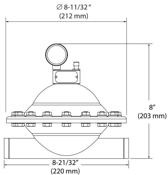
SBP10S-ASS-TA (PASSIVE, 1" NPT THREAD- HORIZONTAL) SBP10S-BSS-TA (PASSIVE, 1" BSP THREAD - HORIZONTAL)
