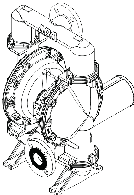
FLANGE MODELS
