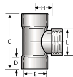
Adapter Tee
