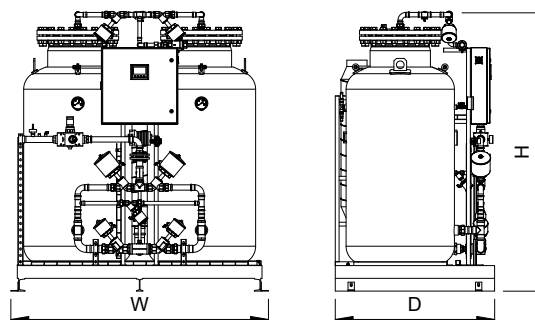
N20 - N150
