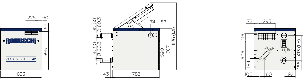
Robox Lobe ES-1.0
