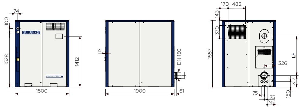
Robox Lobe ES-3.0
