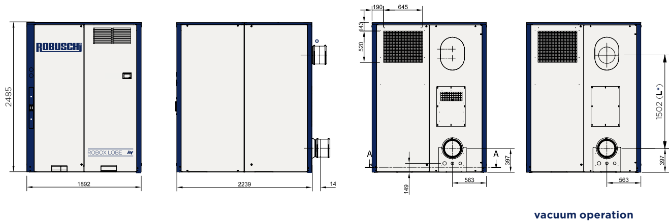
Robox Lobe ES-4.0
