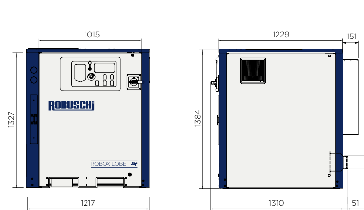
Robox Lobe ES-2.0 PP
