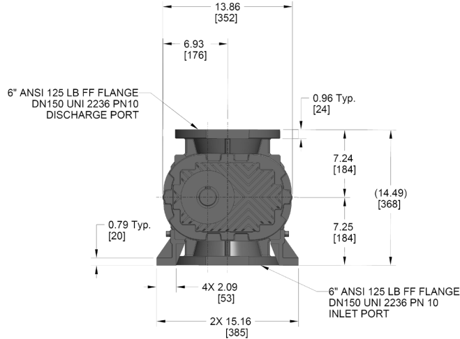
SECTION A-A SCALE 0.750
