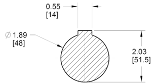
SECTION A-A SCALE 0.750
