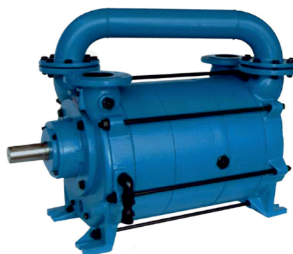
Pumps series TRS Capacity = 10-3500 m 3 /h Vacuum = 200-900 mbar
