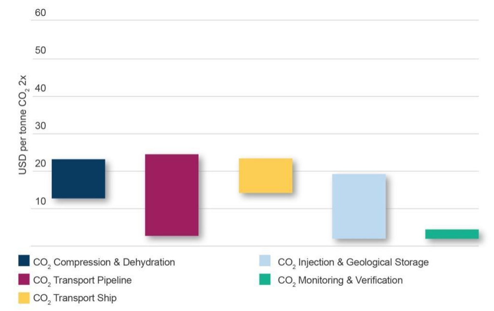
Figure 6: Indicative Costs for CCS Value Chain Components
