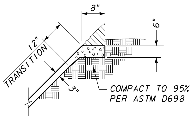
DETAIL ①
