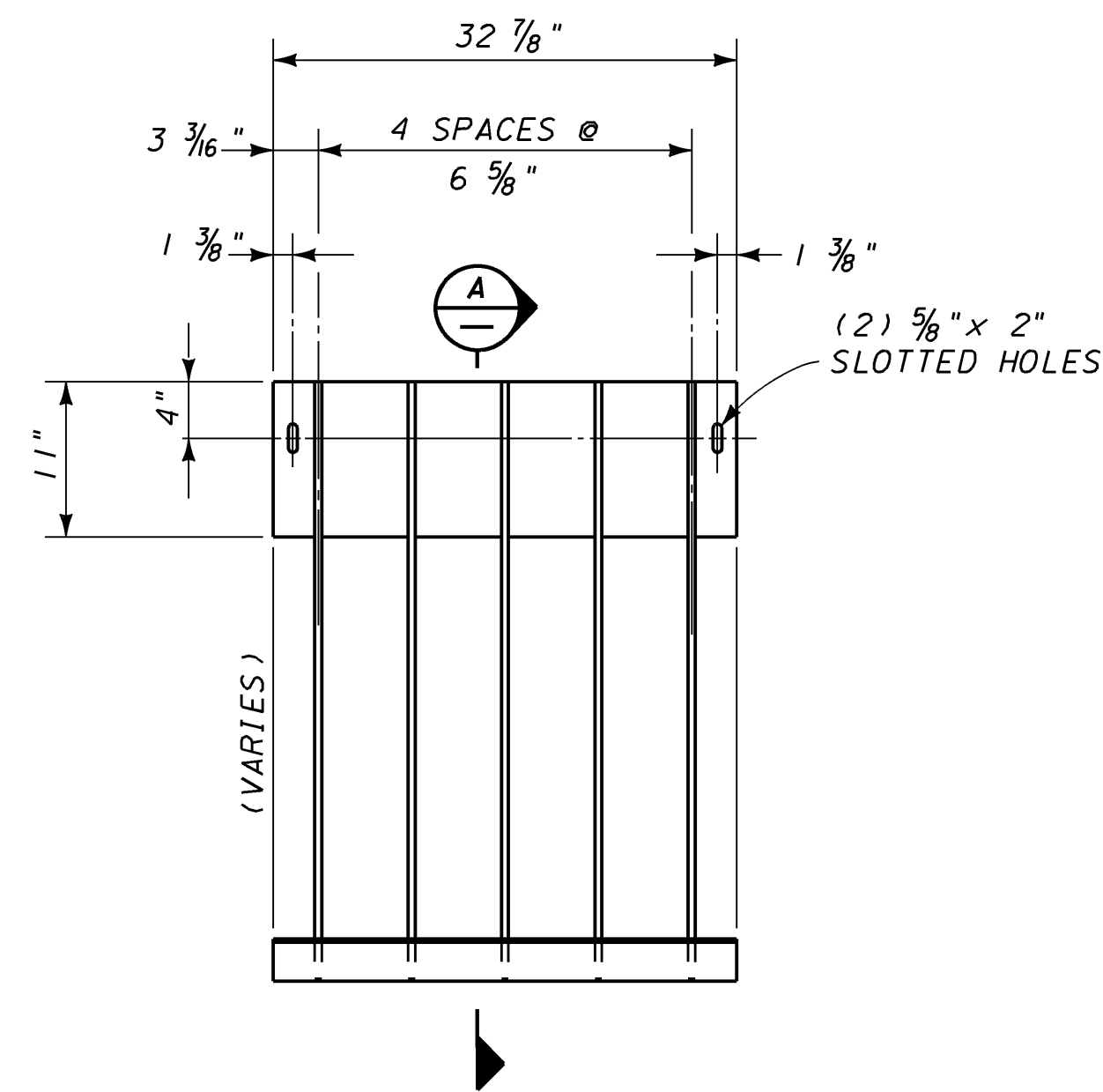
TRASHRACK-TYPE III
