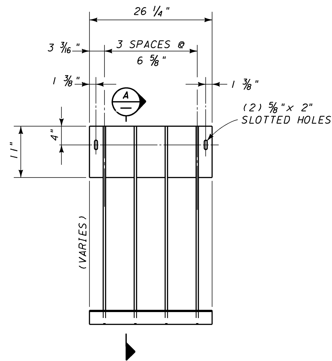
TRASHRACK-TYPE II
