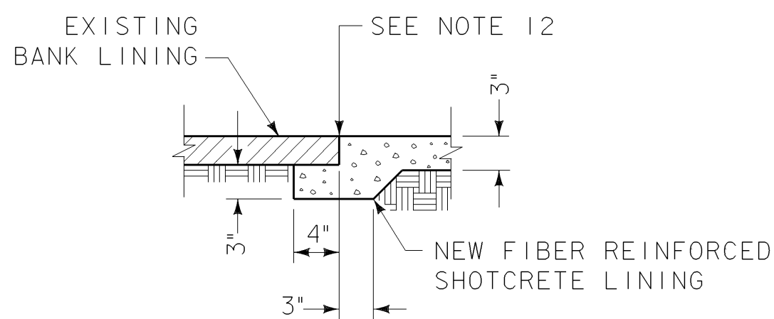
BANK LINING TIE DETAIL ①
