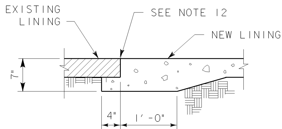
BOTTOM LINING TIE DETAIL ②
