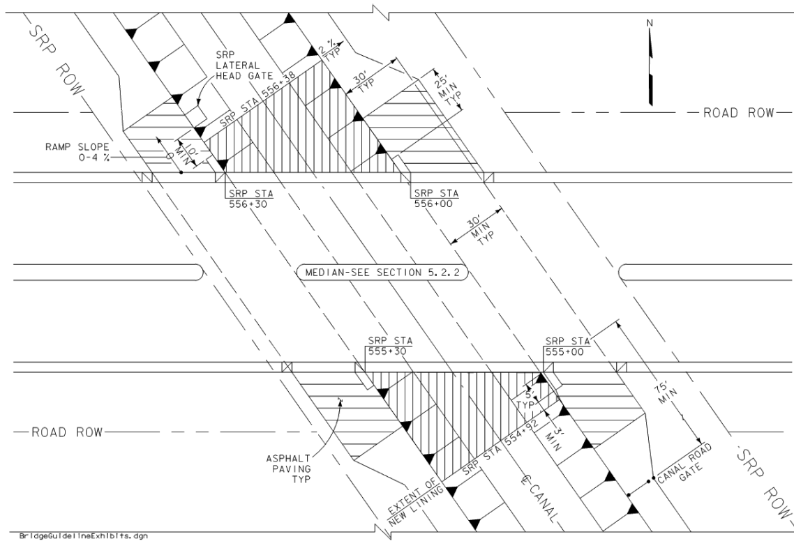
Figure 4 Sample Plan
