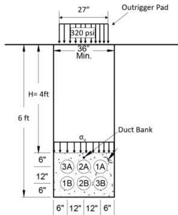
Figure 1. Trench Profile
