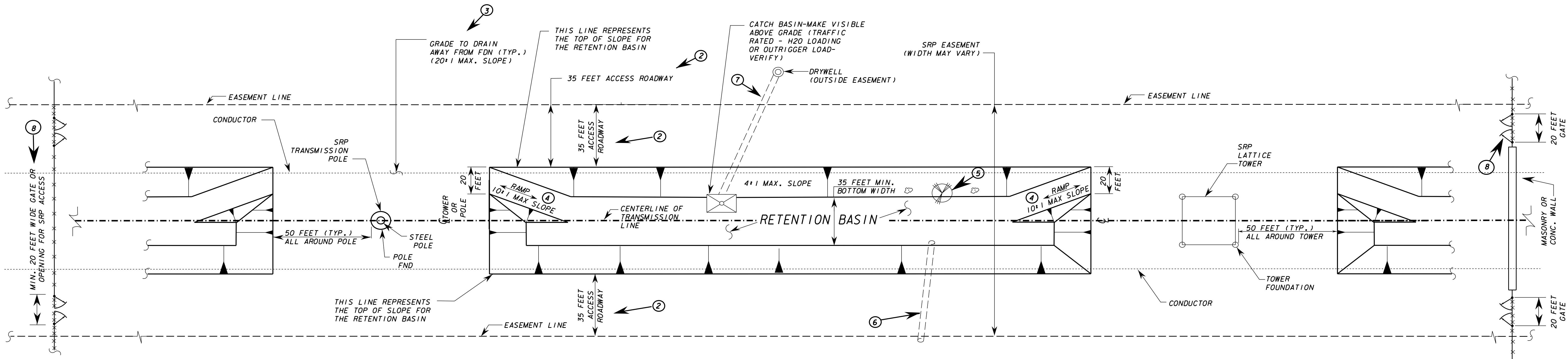
PLAN VIEW OF STORM WATER RETENTION BASIN WITHIN SRP TRANSMISSION LINE RIGHT OF WAY N.T.S.
