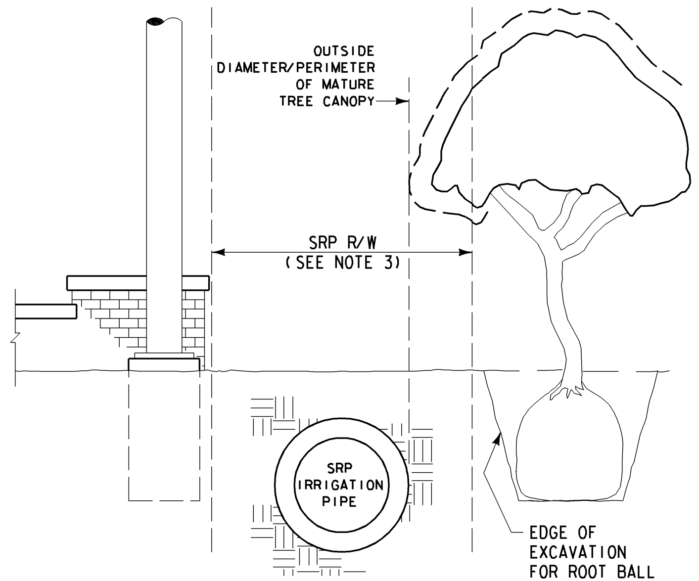
PIPELINES - LANDSCAPING
