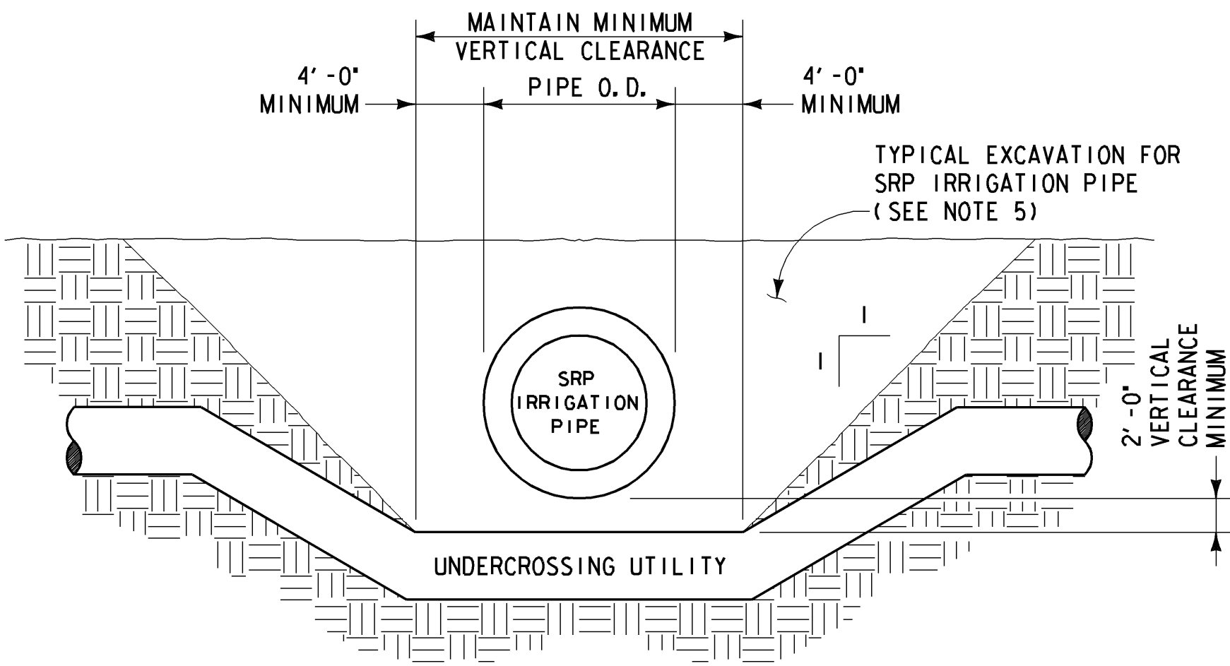
PIPELINE - UNDERCROSSING
