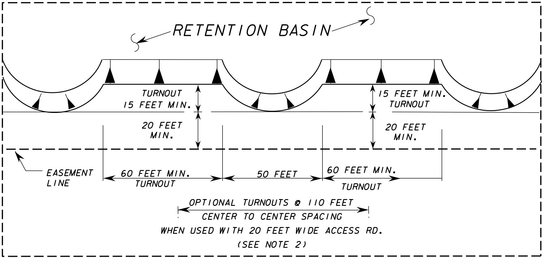
PLAN VIEW OF OPTIONAL TURNOUT @ 110' CENTERS
