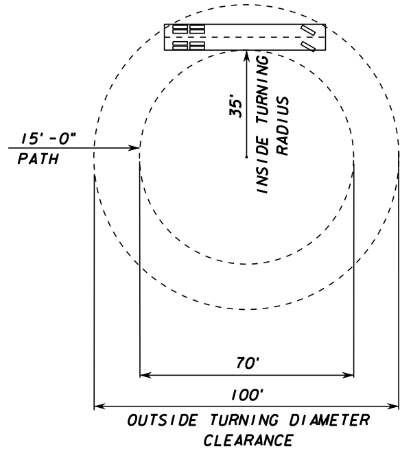
TURNING RADIUS PLAN FOR SRP 69kV MAINTENANCE TRUCK
