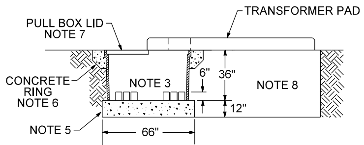
PULL BOX INSTALLED IN ASPHALT PAVEMENT
