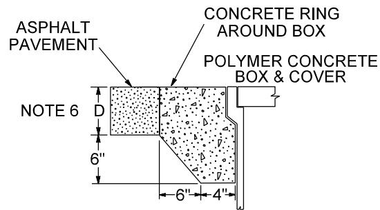
PULL BOX INSTALLED IN ASPHALT PAVEMENT
