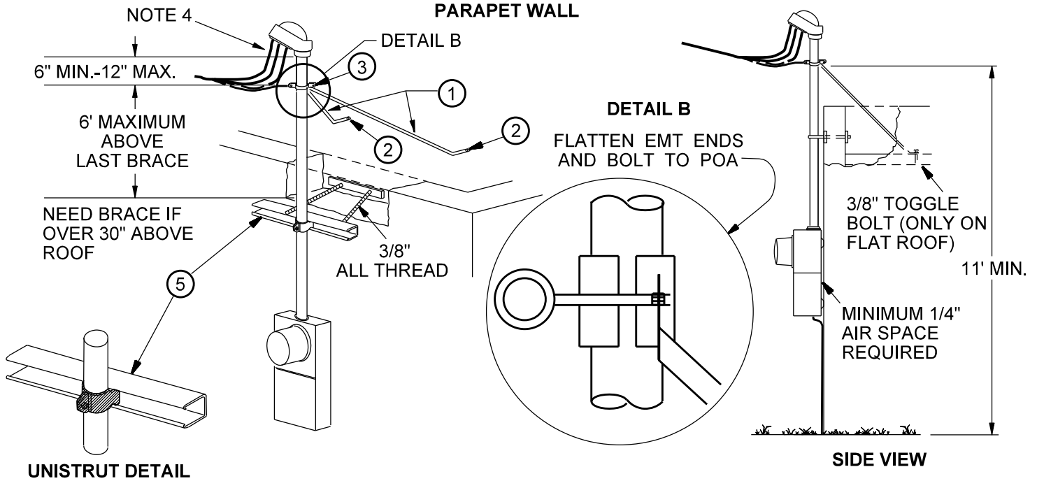
DETAIL A
