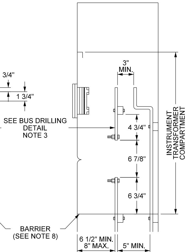
SIDE VIEW
