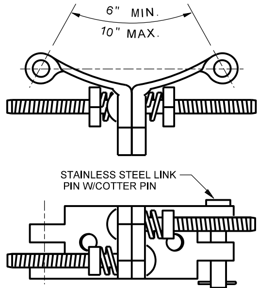
5028488 TAKEUP ASSEMBLY W/PIN
