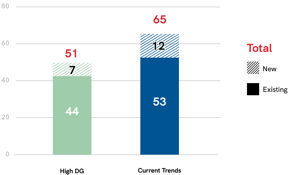
FIGURE 6.42: SUBSTATION BAY ADDITIONS AT EXISTING AND NEW SUBSTATIONS (FY23-35) - HIGH DISTRIBUTED GENERATION SENSITIVITY
