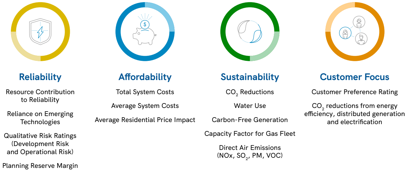
FIGURE 5.18: ISP METRICS
